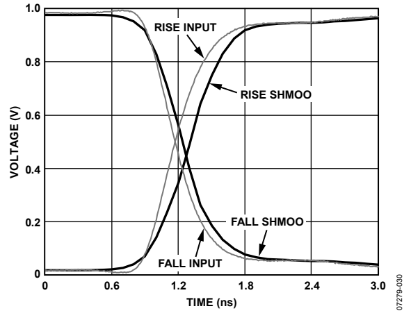
Figure 30. Comparator Shmoo, 1.0 V Input, 0.7 ns (10% to 90%) Input, 50 Ω Terminated
