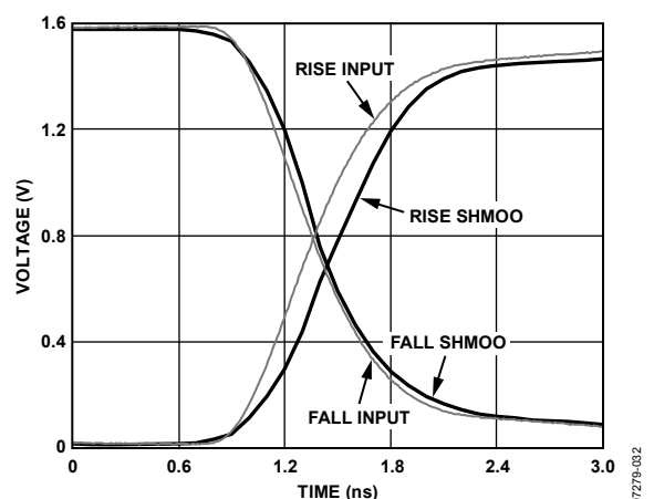
Figure 32. Comparator Shmoo, 1.5 V Input, 1.0 ns (10% to 90%) Input, 50 Ω Terminated
