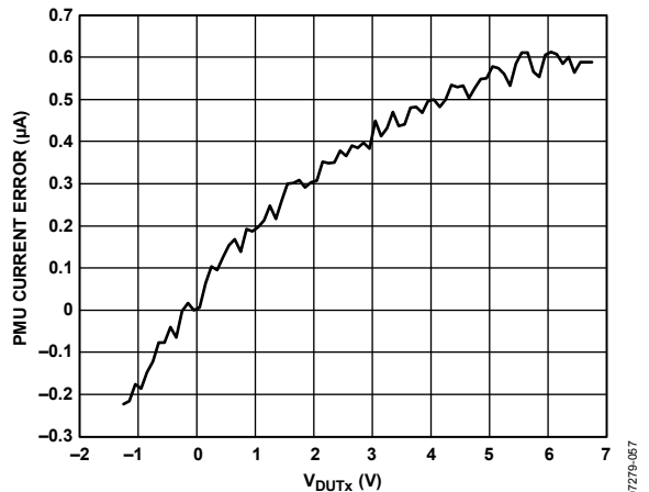
Figure 55. PMU FI Range B Output Current Error at +2\text{ mA} vs. Output Voltage; Output Voltage Is Pulled Externally
